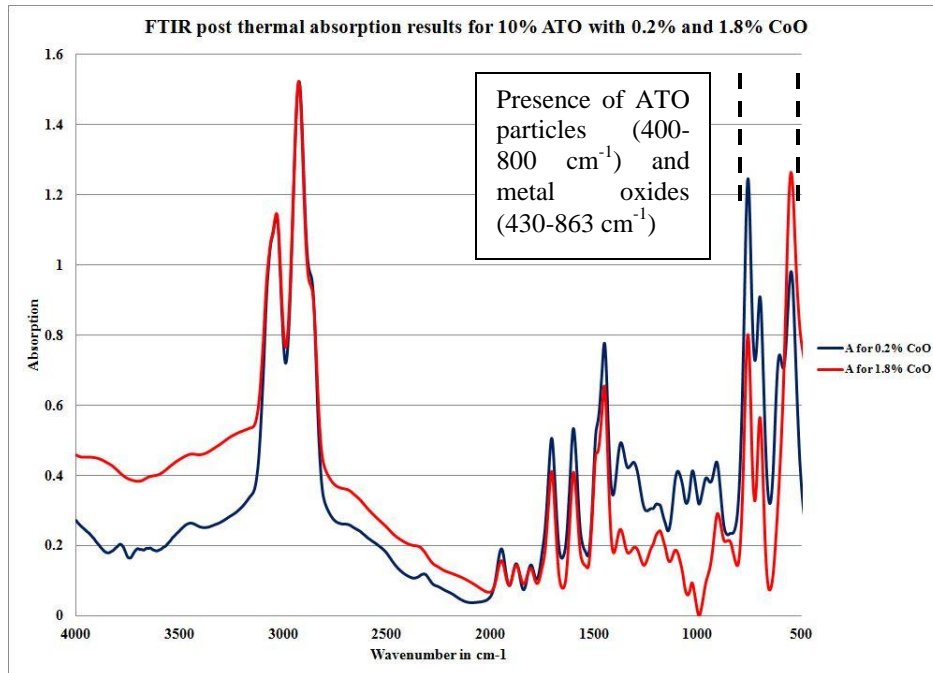
Figure 22: Post thermal FTIR absorption results for 10% ATO with 0.2% and 1.8% CoO
